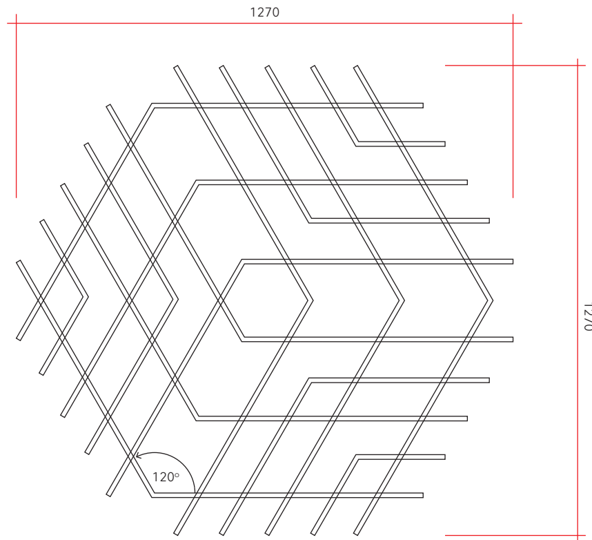
Top view (1 module)
