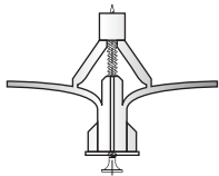
Wing toggle plugs set screw F8 1/2"
