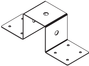
(2) Hanger part, Steel plate Thickness 1.20 mm
