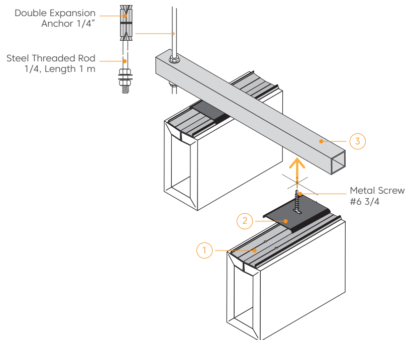
Suspension Expose ceiling
