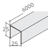
AC 018, U-channel, 1x1", length 6m Color, Aluminum / Mate black
