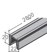
AC 012, PVC Track Profile Lenght 2.80 m, Black Color
