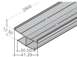
AC-028, for AP12 Beam Baffles Length 2.80m, Aluminum alloy
