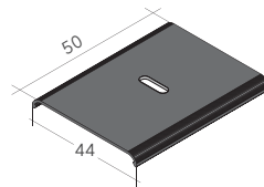
AC-028, for AP12 Beam Baffles Length 2.80m, Aluminum alloy
